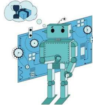
Reinforcement Learning
