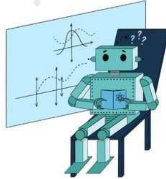
Unsupervised Learning
